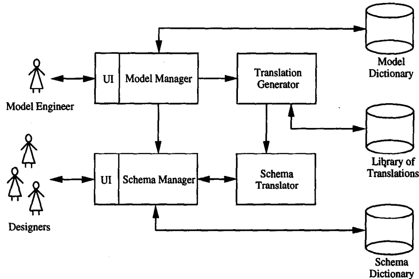
Figure 1: The architecture of the MDM tool
